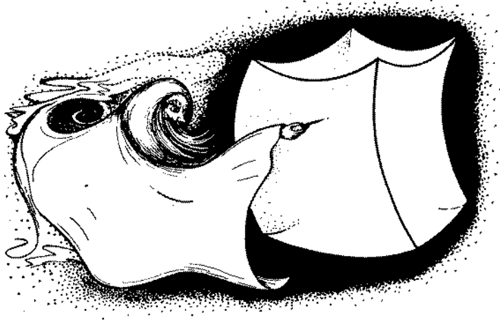
Figure 5. The creator locating the tiny region of phase-space – one part in 10^{10^{123}} – needed to produce a 10^{80} -baryon closed universe with a second law of thermodynamics in the form we know it. From ref. [16]. If the initial state was chosen randomly it would, with overwhelming probability, have led to a universe in a state with maximal entropy. In such a universe there would be no stars, planets, people or a second law.
