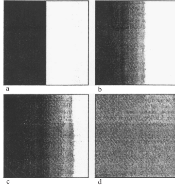
Figure 1. A sequence of “snapshots”, a, b, c, d taken at times t_a, t_b, t_c, t_d , each representing a macroscopic state of a system, say a fluid with two “differently colored” atoms or a solid in which the shading indicates the local temperature. How would you order this sequence in time?
