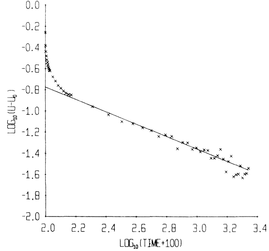
FIG. 12. Energy per site (in units of 2J ) less the equilibrium energy per site as a function of time ( T = 1.10 T_c ). The equation of the straight line, an empirical fit to the data for all but early time, is u - u_0 = 2J \times [2.47(t + 100)^{-7/12}] .
