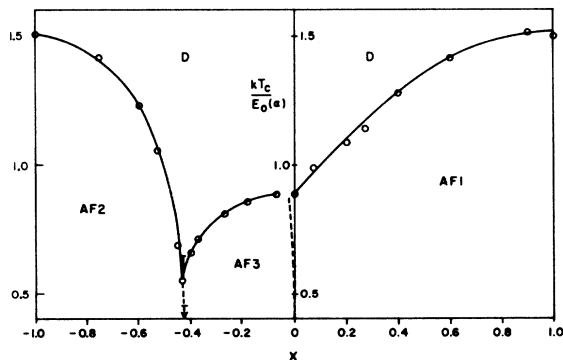
FIG. 2. The T\alpha phase diagram for the fcc lattice, x = 3\alpha/(2+3|\alpha|) . The circles are Monte Carlo data for L=8 except for the point at x= , ( \alpha=-2.0 ). Points at x=\pm 1 are the series of expansion results (Ref. 27). The dashed lines are the proposed boundaries separating the different phases. Close to \alpha=0 and \alpha=-0.5 , the points are triple points, exact location of which cannot be determined.
