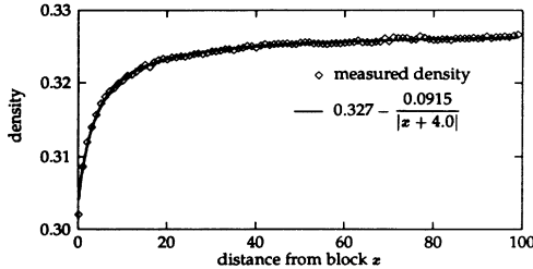
FIG. 2. Density profile near the block, 1200 sites; blockage transmission=0.40; average density=0.5
