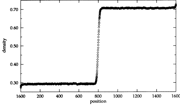
FIG. 1. Density profile, 1600 sites; blockage transmission=0.35; average density=0.5.
