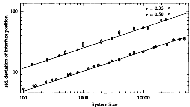
FIG. 4. Interface fluctuations with average density 0.5, r = 0.35, 0.5 . The solid lines have slope \frac{1}{3} .
