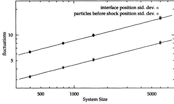
FIG. 6. Fluctuations with uniform (nonrandom) flow through the block. Average density=0.55. Solid lines have slope \frac{1}{3} .
