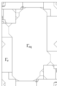
Figure 1: Schematic Picture of the decomposition of \Gamma_E . Here \Gamma_{eq} \equiv \Gamma_{M_{eq}} .
